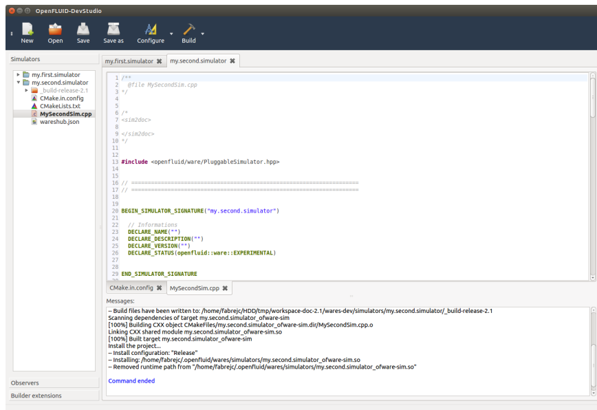
Figure 1.4: Screenshot of OpenFLUID-DevStudio workspace
